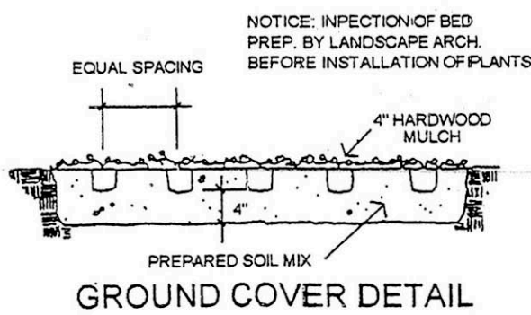
GROUND COVER DETAIL
